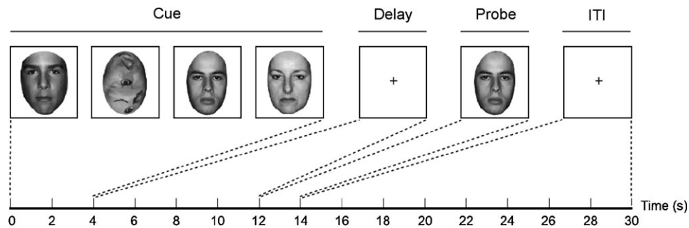
Figure 1. Structure of the behavioral task. On each trial, 4 cue stimuli were serially presented for 1 s each. The stimulus set contained 1, 2, 3, or 4 intact faces, with the remainder of the images (if any) composed of scrambled faces. A trial with a memory load of 3 faces is illustrated here. Participants were instructed to remember all of the intact faces across an 8 s delay period. Following the delay, a probe face appeared for 2 s, and participants made a button press response indicating whether or not the probe face matched any of the cue faces. After responding, participants were instructed to fixate on a crosshair during a 16 s intertrial interval.
