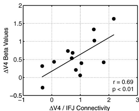
Fig. 5. Correlation between V4 attentional modulation and V4/IFJ functional connectivity. Values represent the difference between attended and ignored color.
